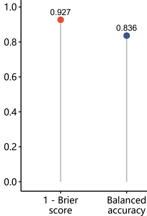
Direction-harmonized score
